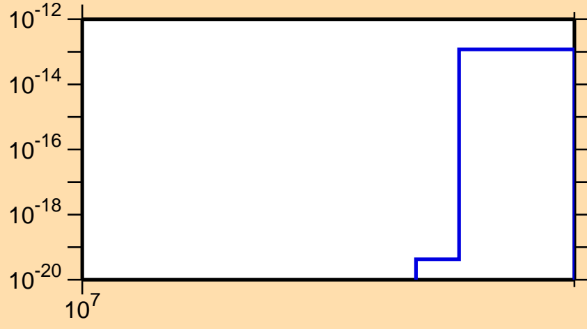
\sigma vs. E for ^{177}\text{Yb}(n,\text{He}3)
