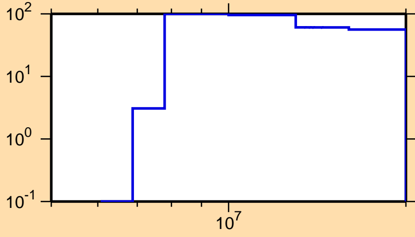
\Delta\sigma/\sigma vs. E for ^{178}\text{Yb}(n,p)
