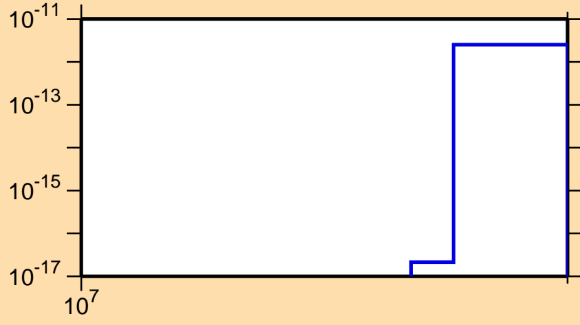
\sigma vs. E for ^{178}\text{Yb}(n,3n\alpha)
