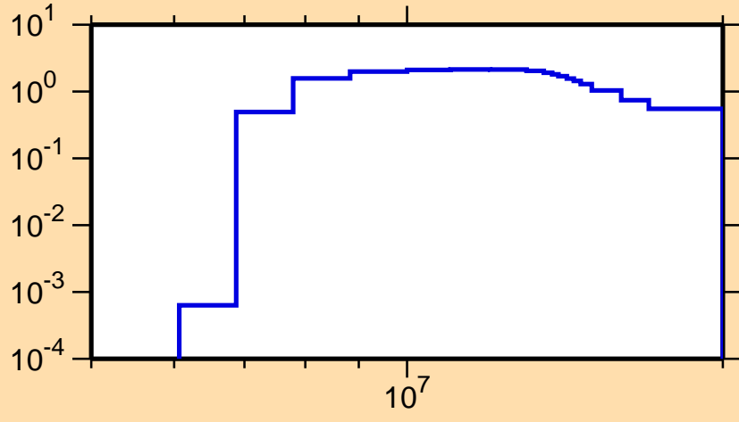
\sigma vs. E for ^{178}\text{Yb}(n,2n)
