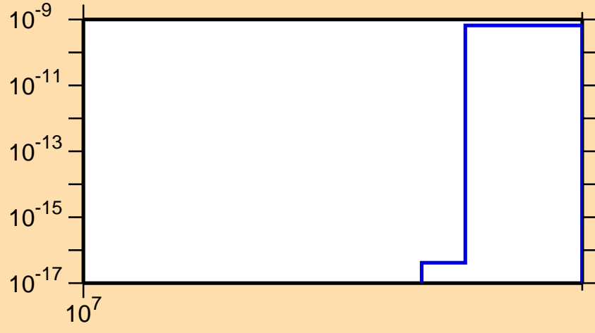
\sigma vs. E for ^{178}\text{Yb}(n,2np)
