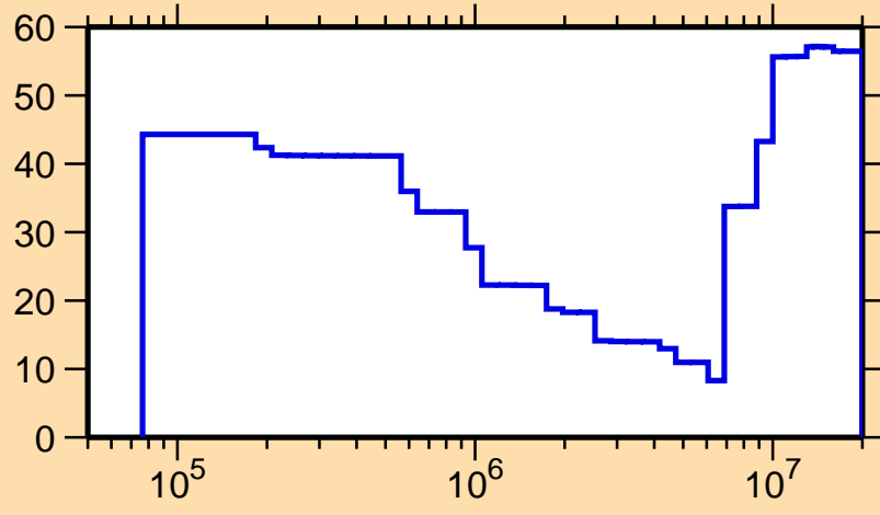
\Delta\sigma/\sigma vs. E for ^{178}\text{Yb}(n,\text{inel.})
