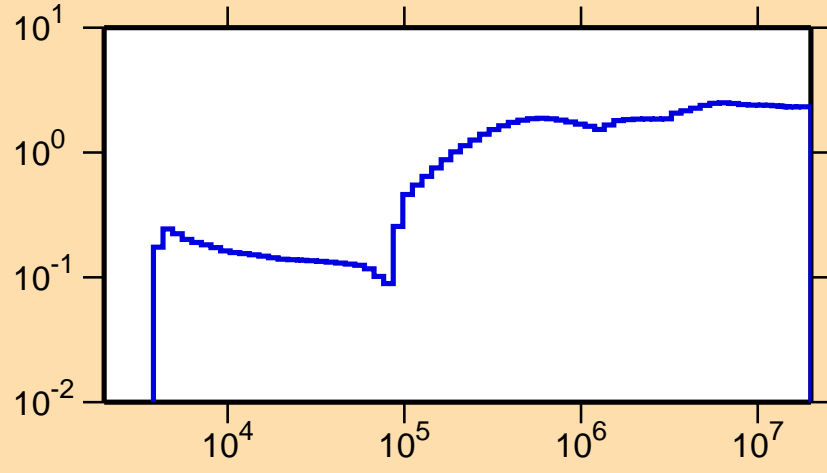
\sigma vs. E for ^{178}\text{Yb}(n,\text{nonel.})
