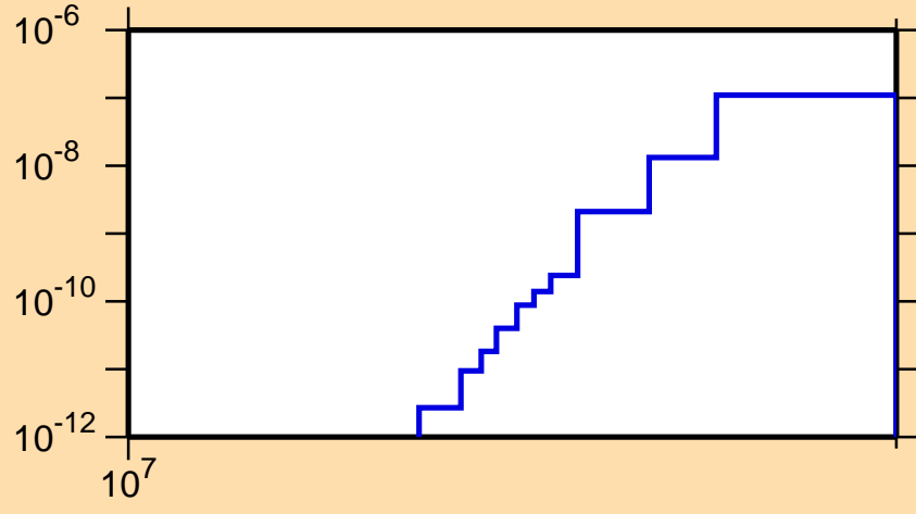
\sigma vs. E for ^{178}\text{Yb}(n,2n\alpha)
