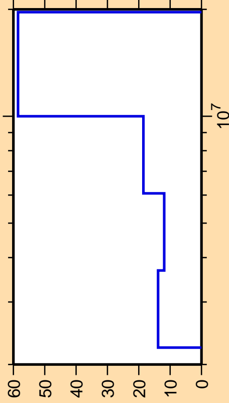
\Delta\sigma/\sigma vs. E for ^{178}\text{Yb}(n, ncont.)
