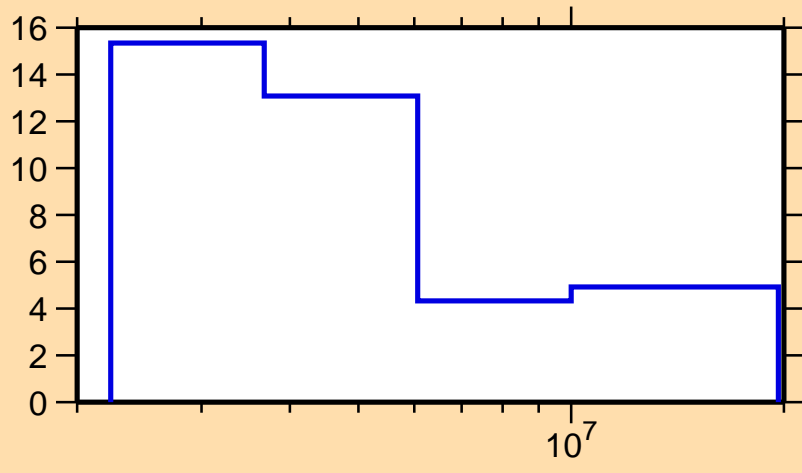
\Delta\sigma/\sigma vs. E for ^{178}\text{Yb}(n, tot.)
