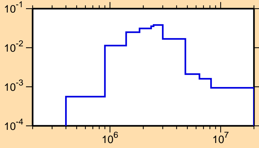
\sigma vs. E for ^{178}\text{Yb}(n,n_3)
