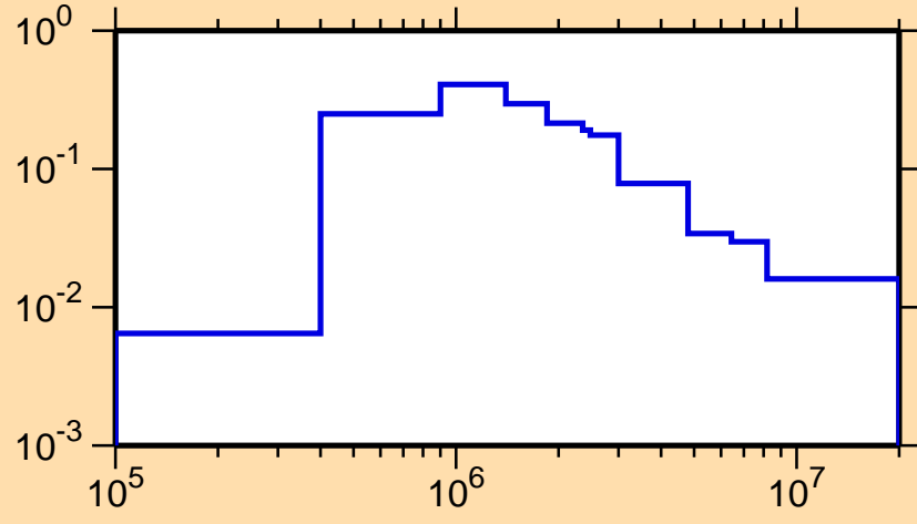
\sigma vs. E for ^{178}\text{Yb}(n,n_2)
