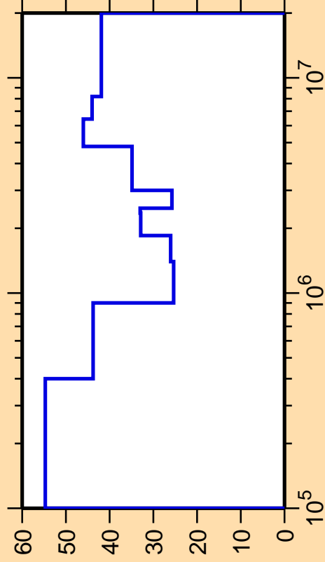
\Delta\sigma/\sigma vs. E for ^{178}\text{Yb}(n,n_2)
