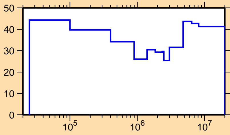
\Delta\sigma/\sigma vs. E for ^{178}\text{Yb}(n,n_1)
