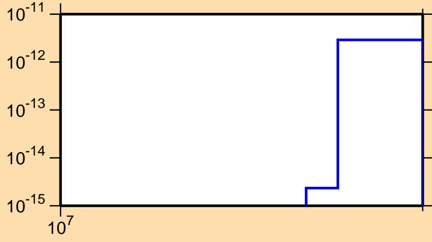
\sigma vs. E for ^{179}\text{Yb}(n,3n\alpha)
