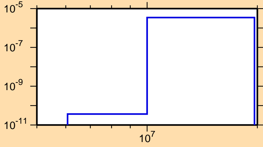
\sigma vs. E for ^{180}\text{Yb}(n,n\alpha)
