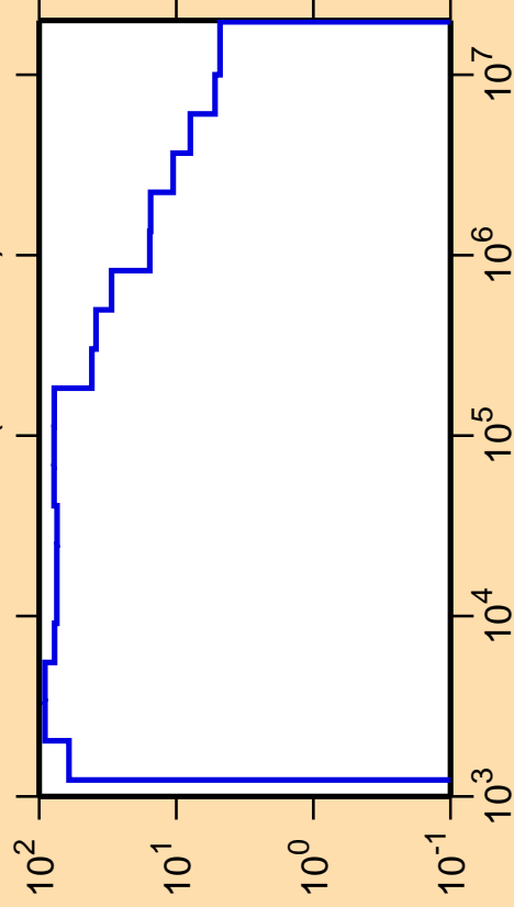
\Delta\sigma/\sigma vs. E for ^{181}\text{Yb}(n,\text{nonel.})
