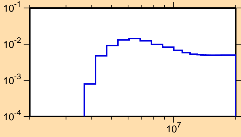
\sigma vs. E for ^{60}\text{Zn}(n,n\text{cont.})
