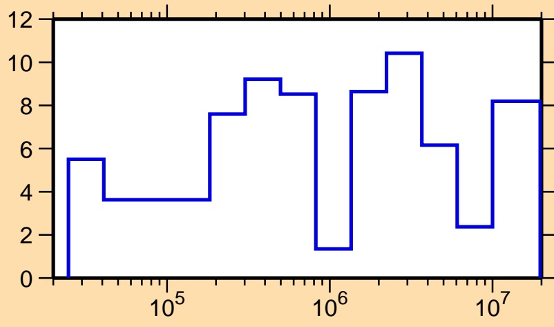
\Delta\sigma/\sigma vs. E for ^{60}\text{Zn}(n,el.)
