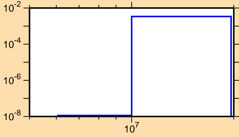
\sigma vs. E for ^{60}\text{Zn}(n,\text{pd})
