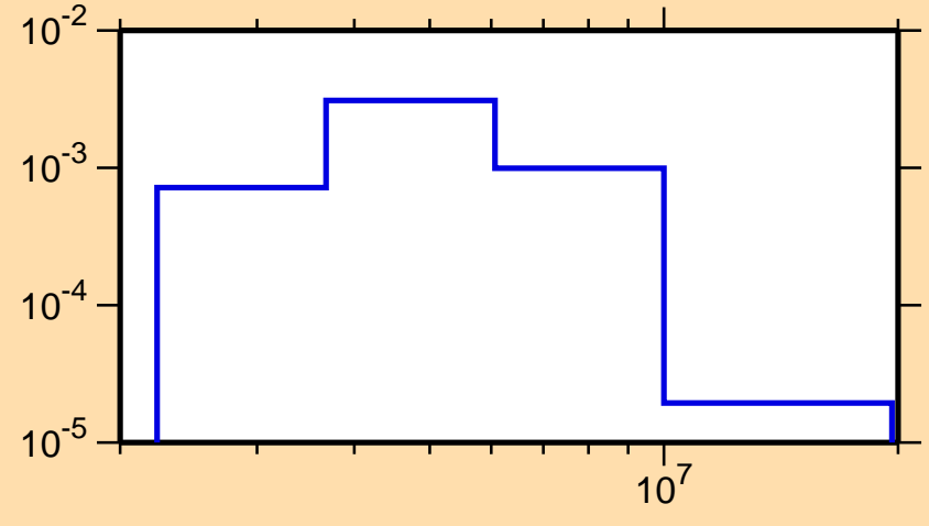
\sigma vs. E for ^{60}\text{Zn}(n,n_4)
