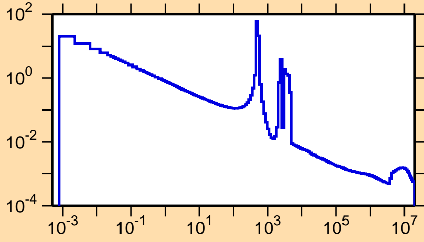
\sigma vs. E for ^{61}\text{Zn}(n,\gamma)
