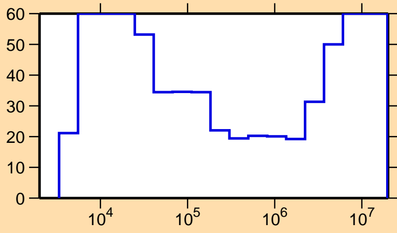
\Delta\sigma/\sigma vs. E for ^{61}\text{Zn}(n,p)
