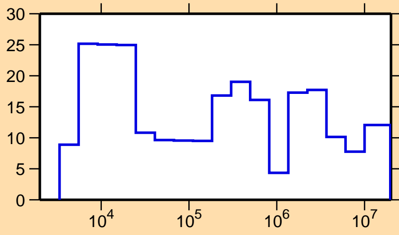
\Delta\sigma/\sigma vs. E for ^{61}\text{Zn}(n,el.)
