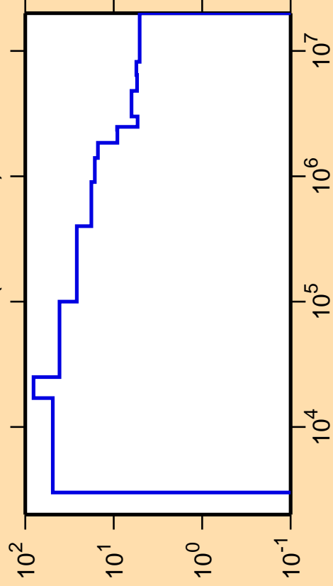
\Delta\sigma/\sigma vs. E for ^{61}\text{Zn}(n,\text{nonel.})
