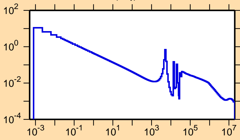
\sigma vs. E for ^{62}\text{Zn}(n,\gamma)
