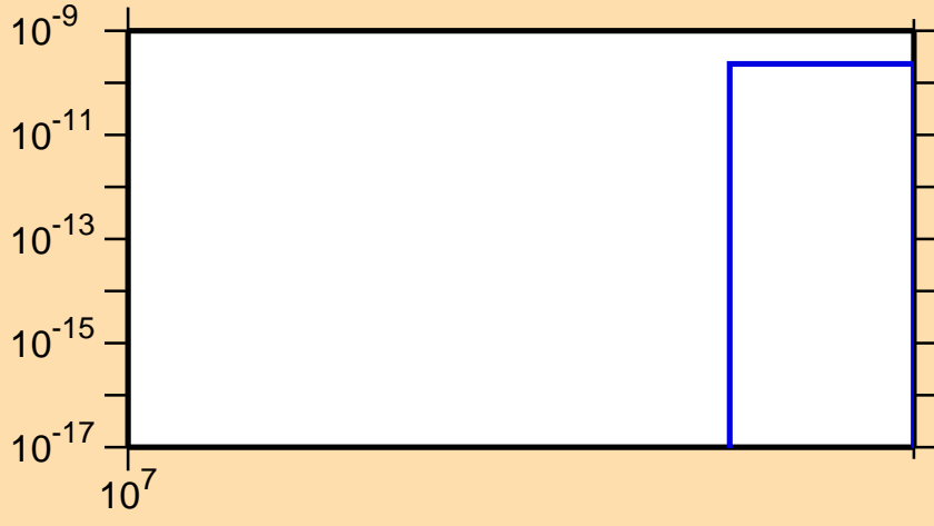
\sigma vs. E for ^{62}\text{Zn} (mt 34)
