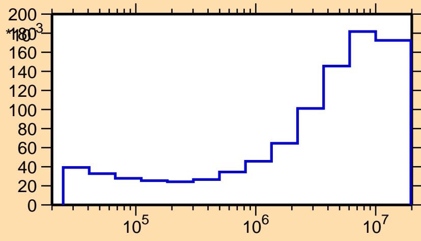
\sigma vs. E for ^{62}\text{Zn}(n,\alpha)
