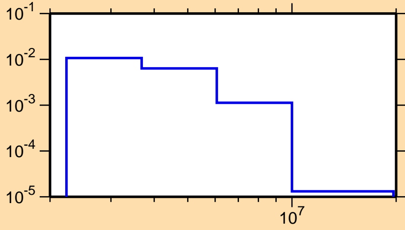
\sigma vs. E for ^{62}\text{Zn}(n,n_4)
