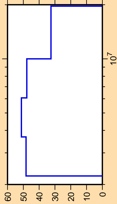
\Delta\sigma/\sigma vs. E for ^{62}\text{Zn}(n,n_4)
