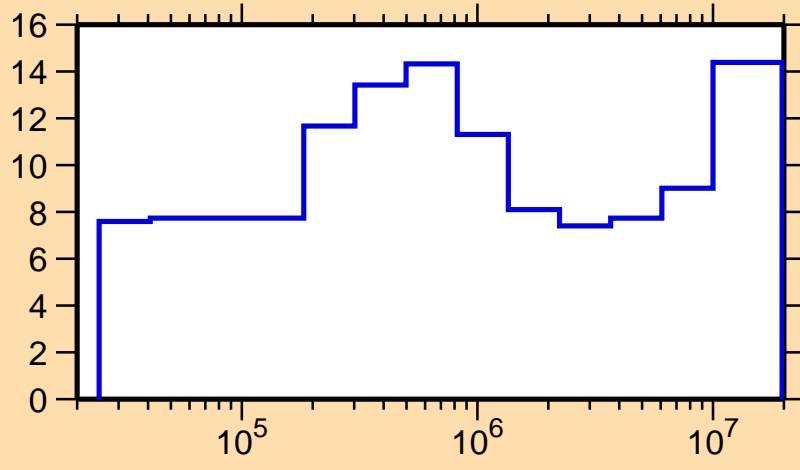
\Delta\sigma/\sigma vs. E for ^{62}\text{Zn}(n,el.)
