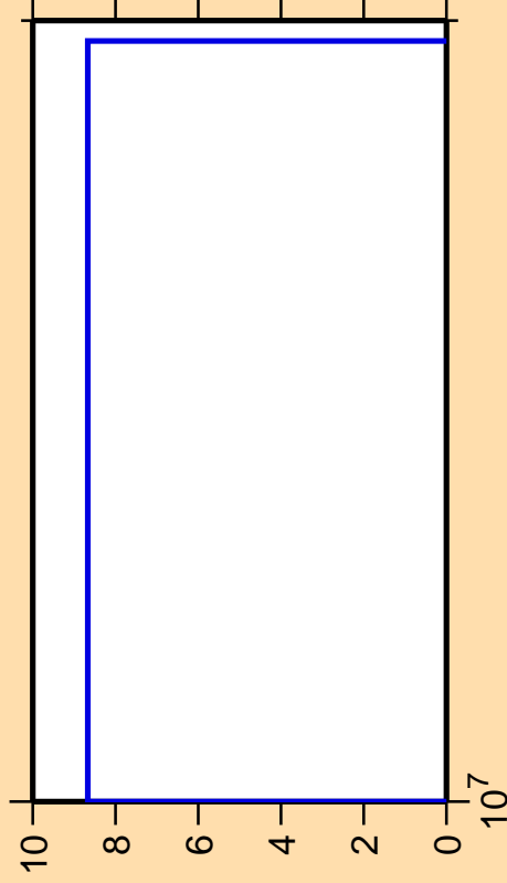
\Delta\sigma/\sigma vs. E for ^{62}\text{Zn} (mt 34)
