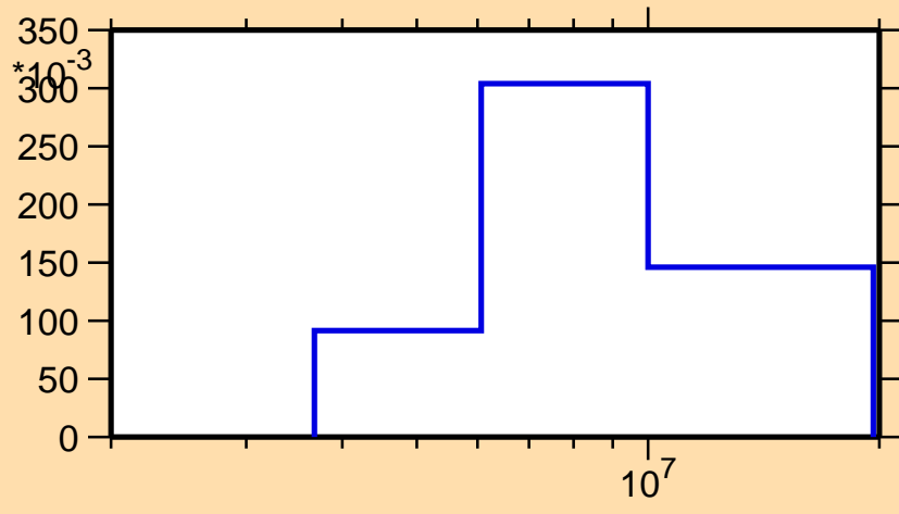
\sigma vs. E for ^{62}\text{Zn}(n,n\text{cont.})
