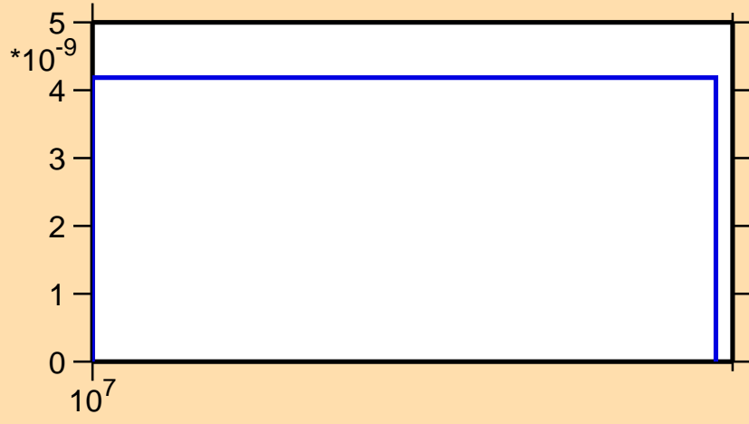
\sigma vs. E for ^{62}\text{Zn} (mt 45)
