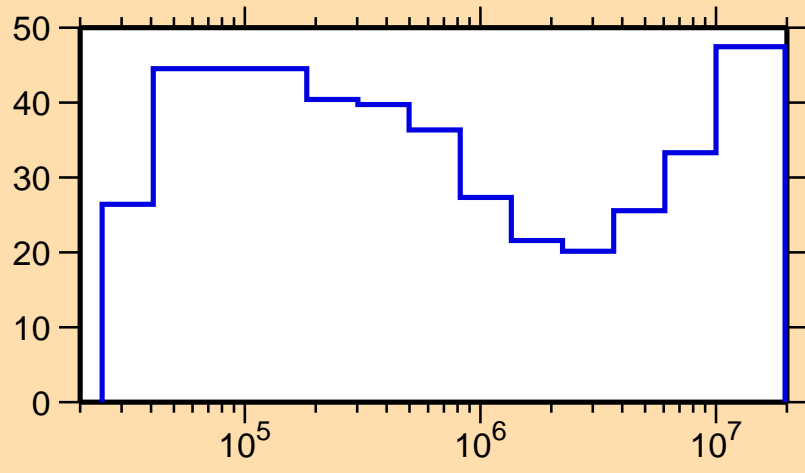
\Delta\sigma/\sigma vs. E for ^{62}\text{Zn}(n,p)
