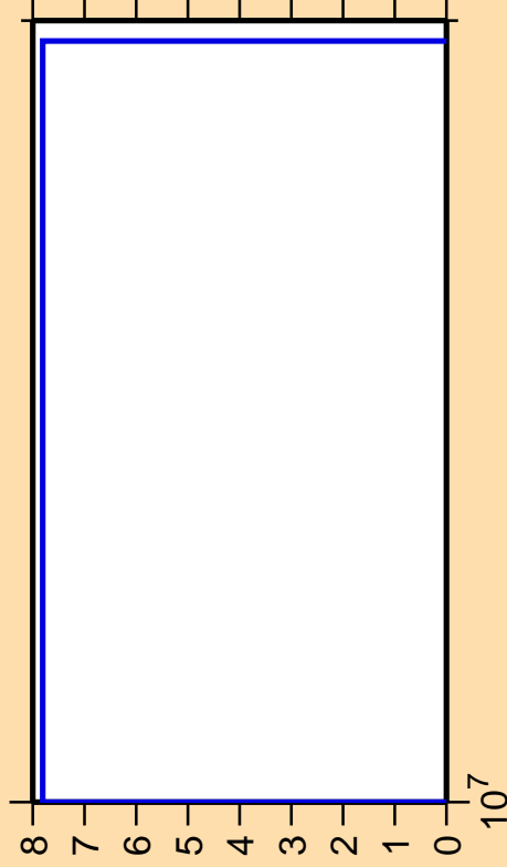
\Delta\sigma/\sigma vs. E for ^{62}\text{Zn}(n,2n\alpha)
