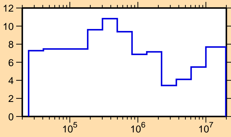
\Delta\sigma/\sigma vs. E for ^{62}\text{Zn}(n,\text{tot.})
