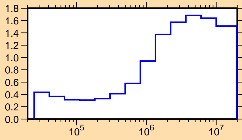
\sigma vs. E for ^{62}\text{Zn}(n,\text{nonel.})
