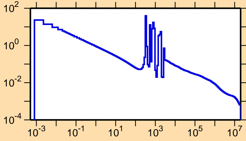
\sigma vs. E for ^{63}\text{Zn}(n,\gamma)
