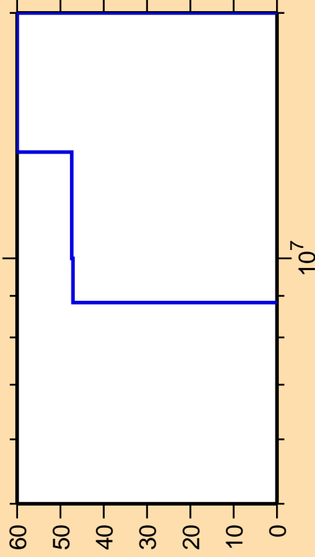
\Delta\sigma/\sigma vs. E for ^{63}\text{Zn}(n,2n)
