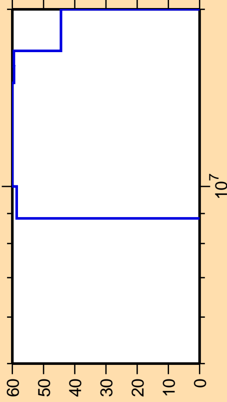
\Delta\sigma/\sigma vs. E for ^{63}\text{Zn}(n,n_{\text{cont}}) .
