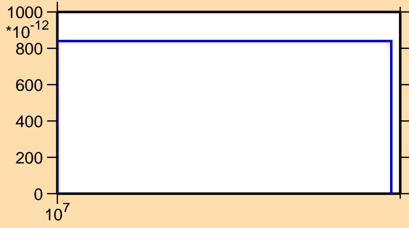
\sigma vs. E for ^{63}\text{Zn} (mt 34)
