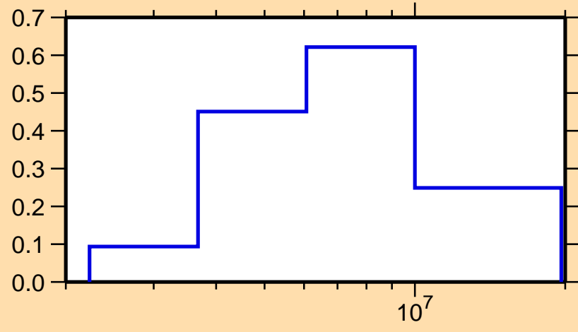
\sigma vs. E for ^{63}\text{Zn}(n,n\text{cont.})
