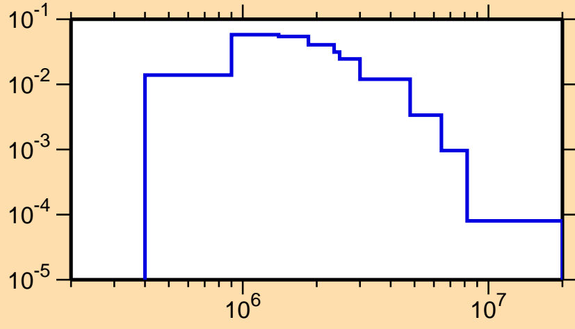
\sigma vs. E for ^{63}\text{Zn}(n,n_3)
