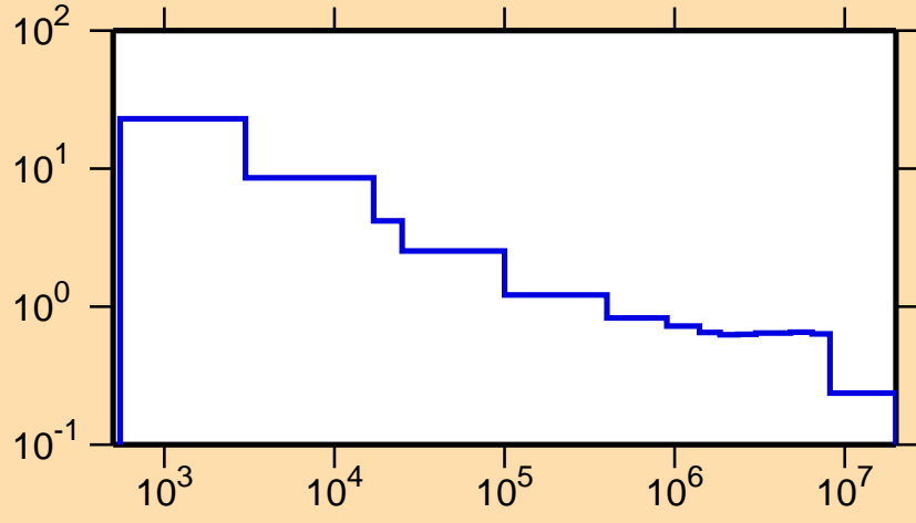
\sigma vs. E for ^{63}\text{Zn}(n,p)
