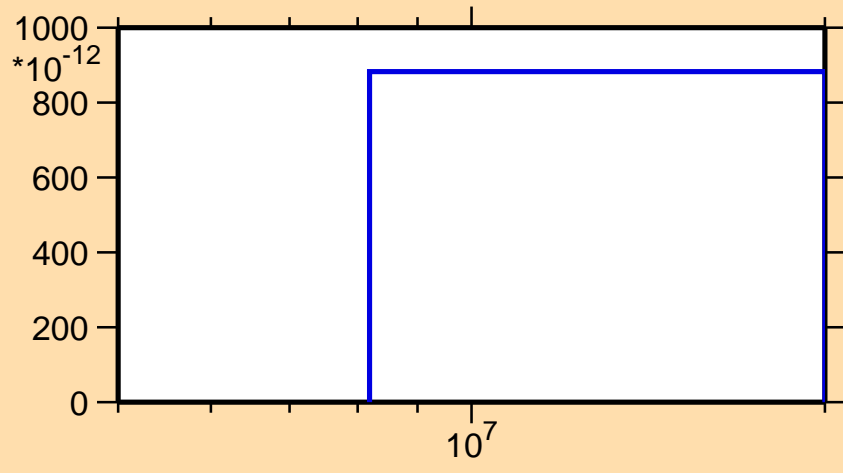
\sigma vs. E for ^{63}\text{Zn} (mt 34)
