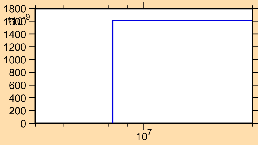
\sigma vs. E for ^{63}\text{Zn}(n,\text{nd})
