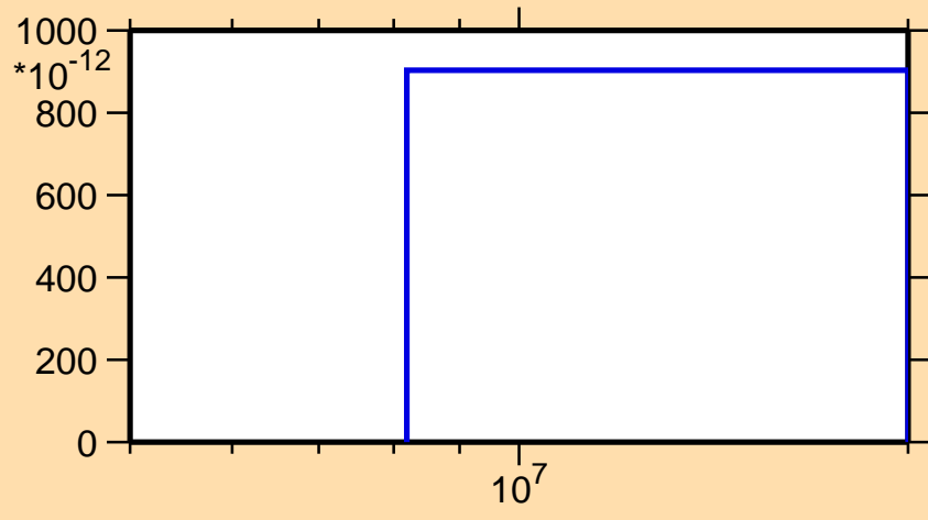
\sigma vs. E for ^{63}\text{Zn}(\text{mt117})
