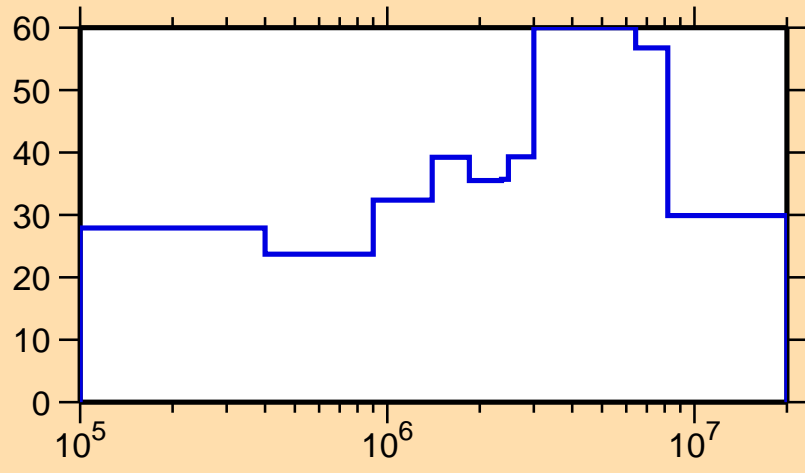
\Delta\sigma/\sigma vs. E for ^{63}\text{Zn}(n,n_1)
