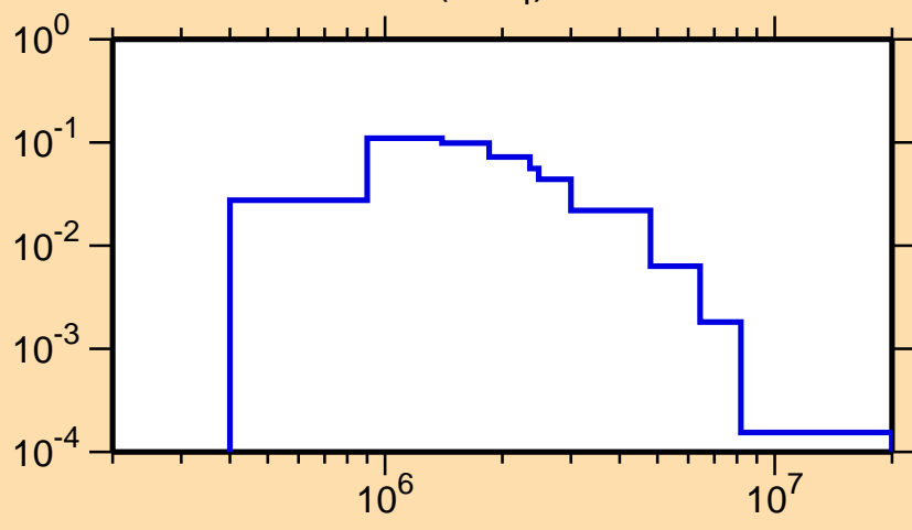
\sigma vs. E for ^{63}\text{Zn}(n,n_4)
