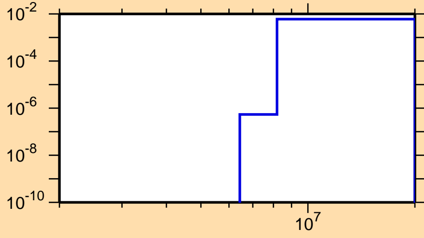
\sigma vs. E for ^{63}\text{Zn}(n,p\alpha)
