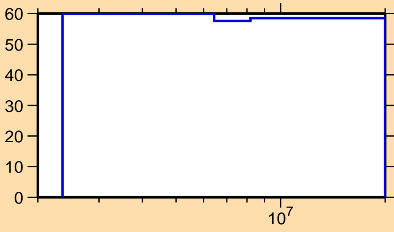
\Delta\sigma/\sigma vs. E for ^{63}\text{Zn}(n,n\text{cont.})
