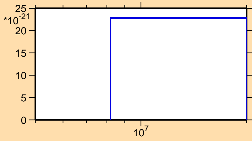
\sigma vs. E for ^{63}\text{Zn}(n,nt)
