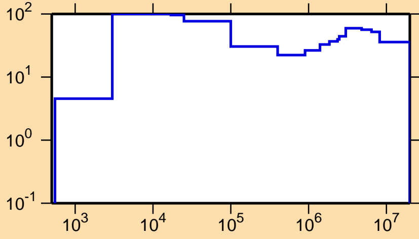
\Delta\sigma/\sigma vs. E for ^{63}\text{Zn}(n,p)
