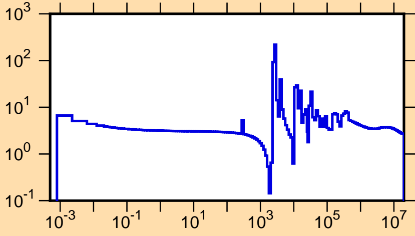
\sigma vs. E for ^{64}\text{Zn}(n,\text{tot.})
