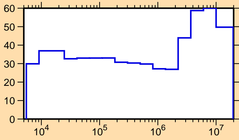
\Delta\sigma/\sigma vs. E for ^{65}\text{Zn}(n,p)
