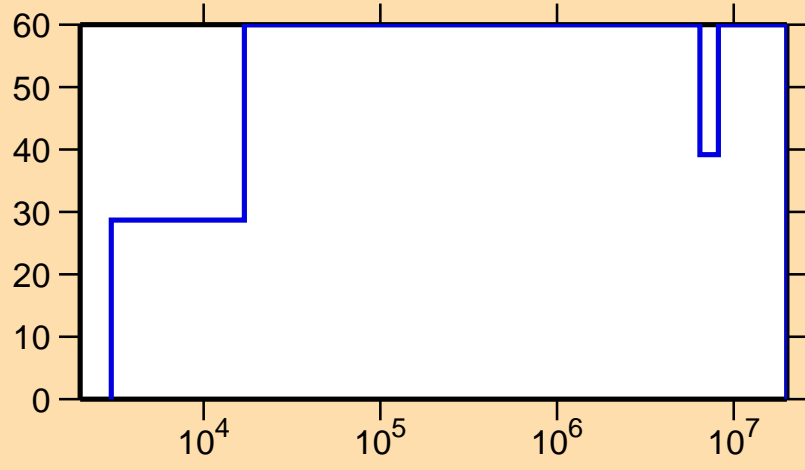
\Delta\sigma/\sigma vs. E for ^{65}\text{Zn}(n,\gamma)
