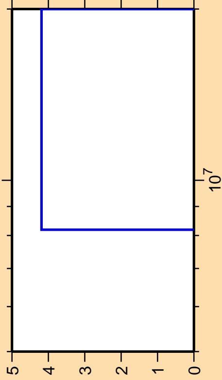
\Delta\sigma/\sigma vs. E for ^{65}\text{Zn}(\text{mt117})
