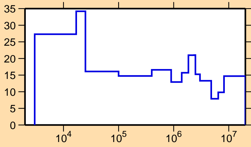
\Delta\sigma/\sigma vs. E for ^{65}\text{Zn}(n,el.)
