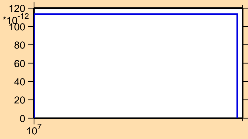
\sigma vs. E for ^{66}\text{Zn}(n,2n\alpha)
