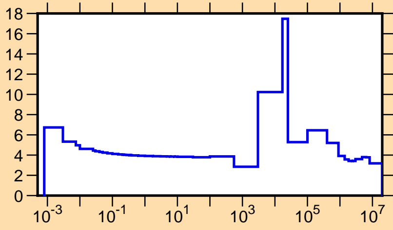
\sigma vs. E for ^{66}\text{Zn}(n,\text{tot.})
