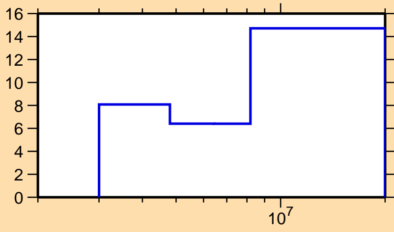
\Delta\sigma/\sigma vs. E for ^{66}\text{Zn}(n,ncont.)
