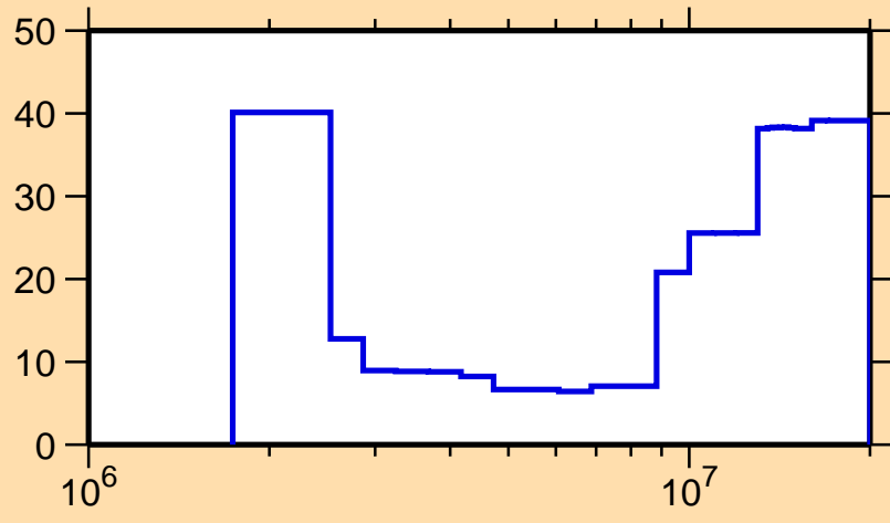
\Delta\sigma/\sigma vs. E for ^{67}\text{Zn}(n,ncont.)
