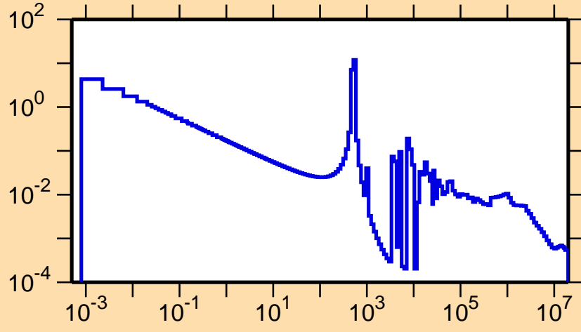
\sigma vs. E for ^{68}\text{Zn}(n,\gamma)
