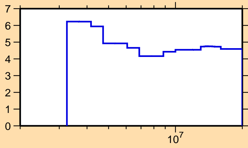
\Delta\sigma/\sigma vs. E for ^{68}\text{Zn}(n,n\text{onel.})
