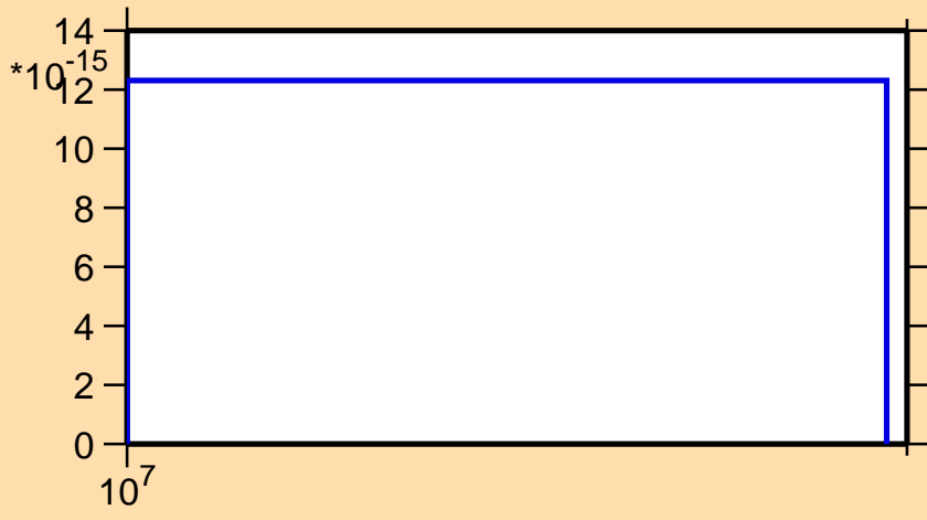
\sigma vs. E for ^{68}\text{Zn}(n,p\alpha)
