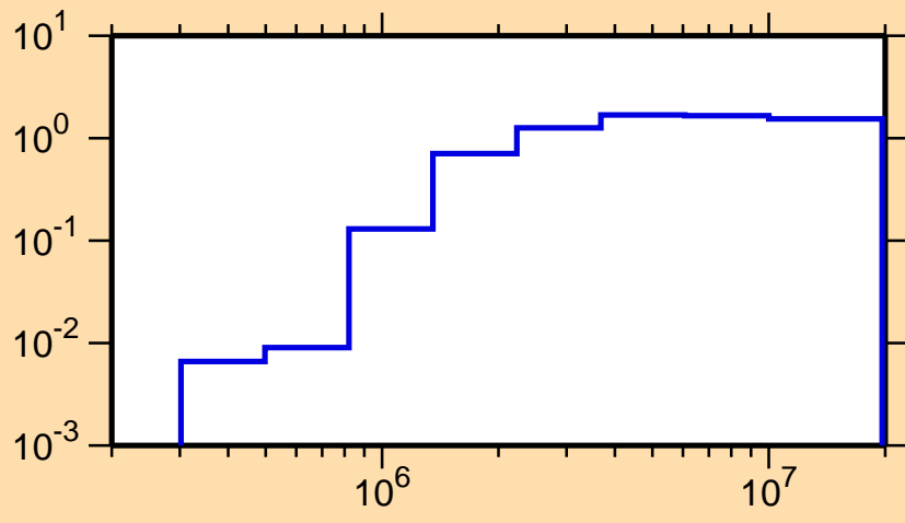
\sigma vs. E for ^{68}\text{Zn}(n,\text{nonel.})
