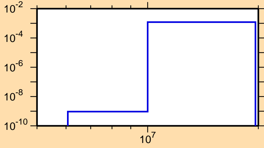
\sigma vs. E for ^{68}\text{Zn}(n,d)
