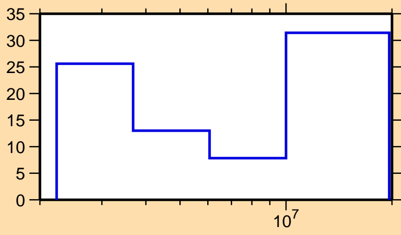
\Delta\sigma/\sigma vs. E for ^{68}\text{Zn}(n,n\text{cont.})
