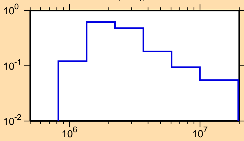
\sigma vs. E for ^{68}\text{Zn}(n,n_1)
