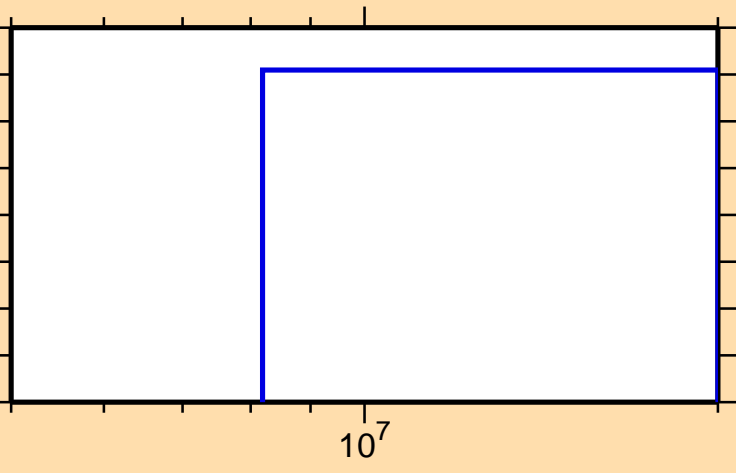
\sigma vs. E for ^{68}\text{Zn}(n,3n)
