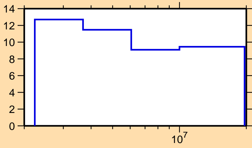
\Delta\sigma/\sigma vs. E for ^{69}\text{Zn}(n,n\text{onel.})
