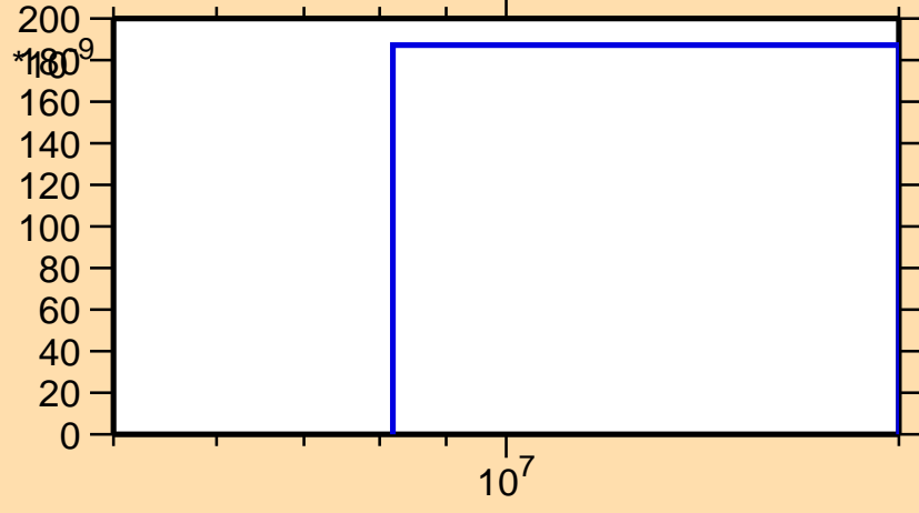
\sigma vs. E for ^{69}\text{Zn}(n,nd)
