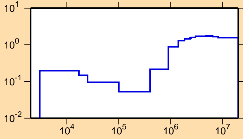
\sigma vs. E for ^{69}\text{Zn}(n,\text{nonel.})
