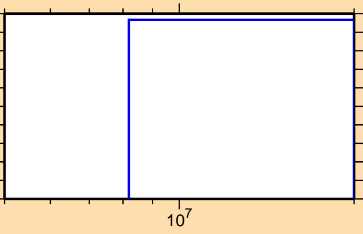
\sigma vs. E for ^{69}\text{Zn}(n,2np)
