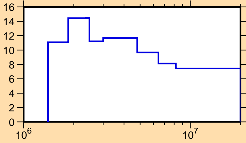
\Delta\sigma/\sigma vs. E for ^{69}\text{Zn}(n,n\text{onel.})
