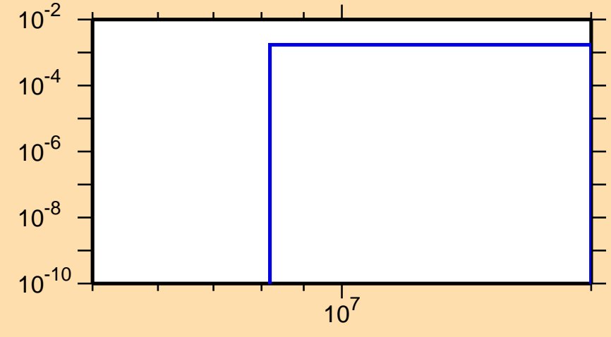
\sigma vs. E for ^{69}\text{Zn}(n,n\alpha)
