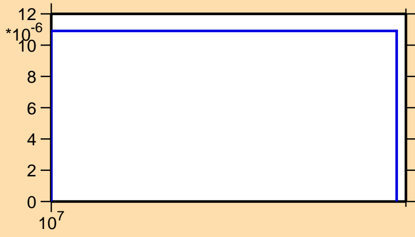
\sigma vs. E for ^{70}\text{Zn}(n,t)
