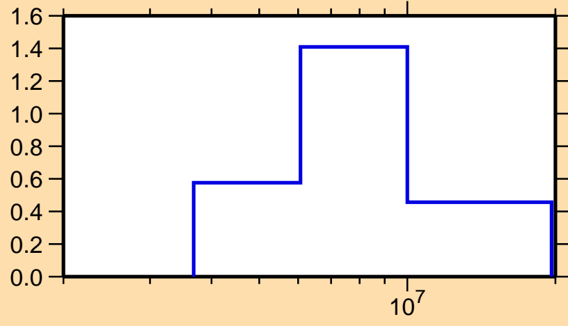
\sigma vs. E for ^{70}\text{Zn}(n,n\text{cont.})
