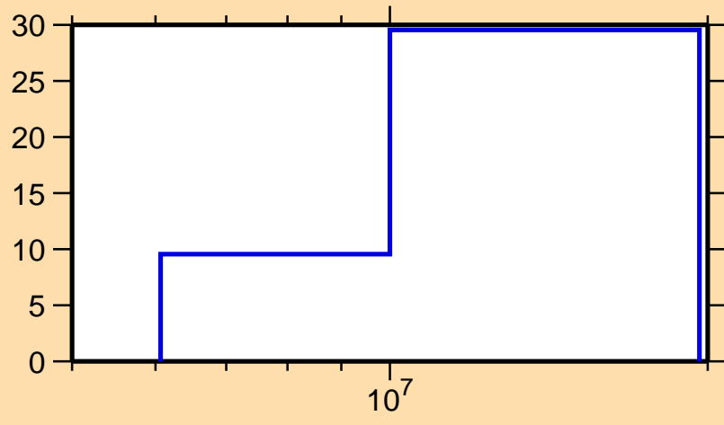
\Delta\sigma/\sigma vs. E for ^{70}\text{Zn}(n,ncont.)
