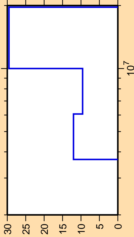
\Delta\sigma/\sigma vs. E for ^{70}\text{Zn}(n,n\text{cont.})
