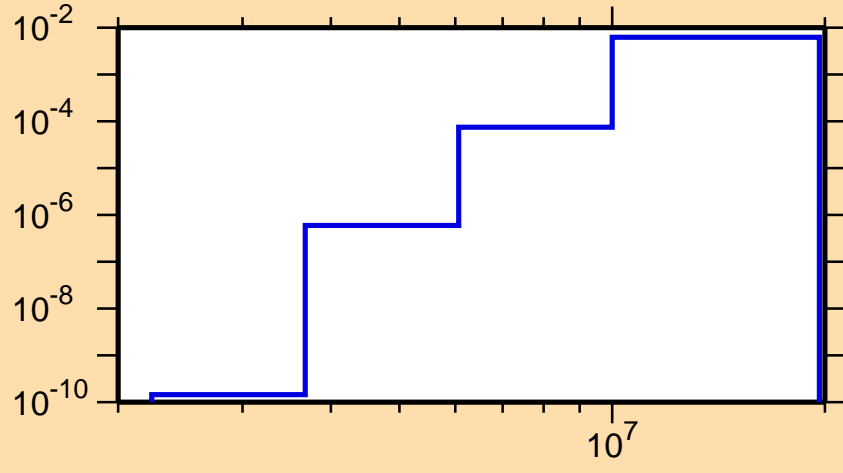
\sigma vs. E for ^{70}\text{Zn}(n,\alpha)
