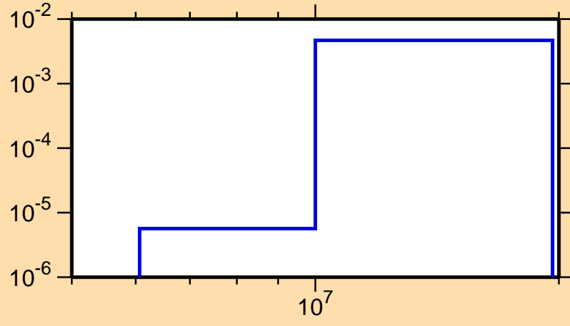
\sigma vs. E for ^{70}\text{Zn}(n,p)
