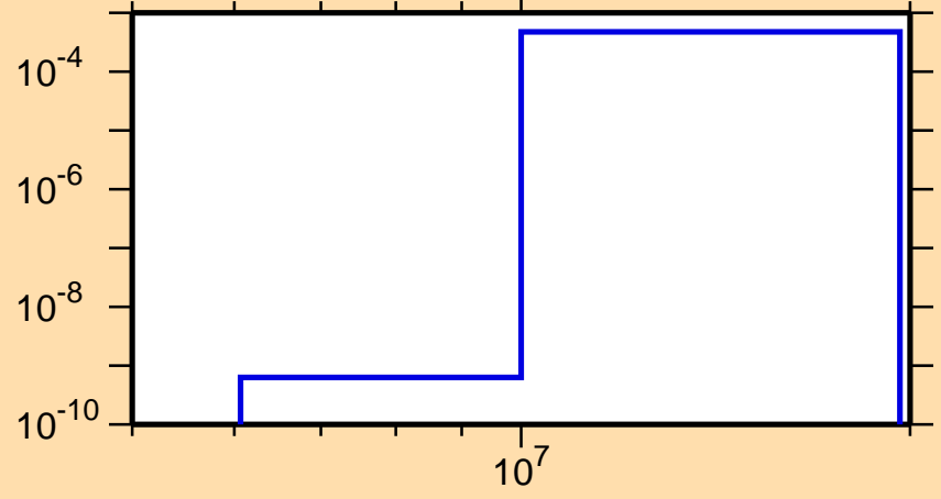
\sigma vs. E for ^{70}\text{Zn}(n,n\alpha)
