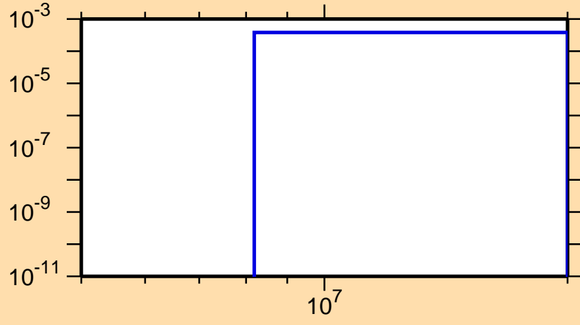
\sigma vs. E for ^{70}\text{Zn}(n,n\alpha)
