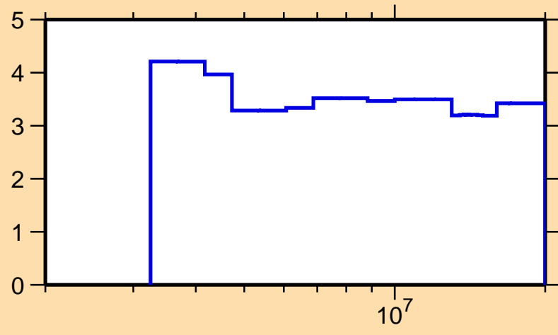
\Delta\sigma/\sigma vs. E for ^{71}\text{Zn}(n,n\text{onrel.})
