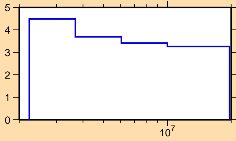
\Delta\sigma/\sigma vs. E for ^{71}\text{Zn}(n,n\text{onel.})
