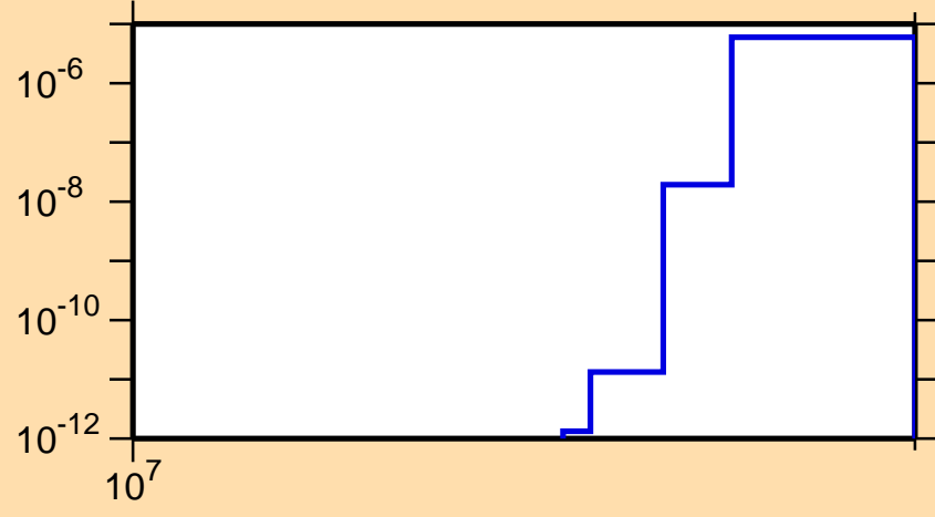
\sigma vs. E for ^{71}\text{Zn}(n,nd)
