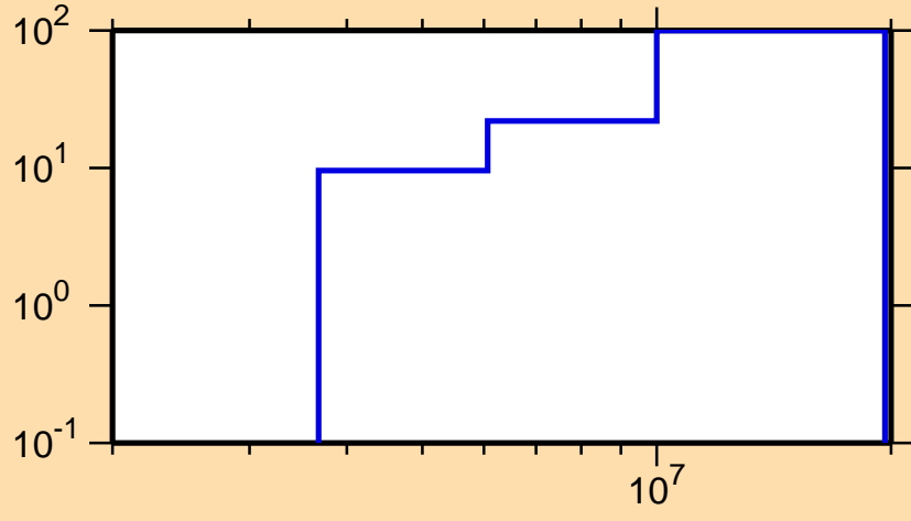
\Delta\sigma/\sigma vs. E for ^{71}\text{Zn}(n,ncont.)
