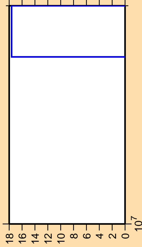
\Delta\sigma/\sigma vs. E for ^{72}\text{Zn}(n,nd)
