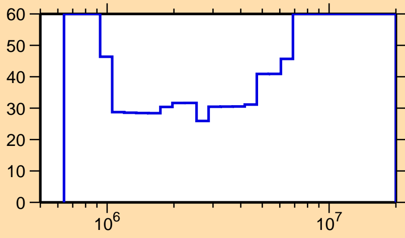
\Delta\sigma/\sigma vs. E for ^{72}\text{Zn}(n,n_1)
