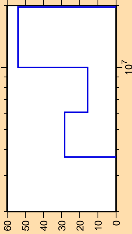
\Delta\sigma/\sigma vs. E for ^{72}\text{Zn}(n,n\text{cont.})
