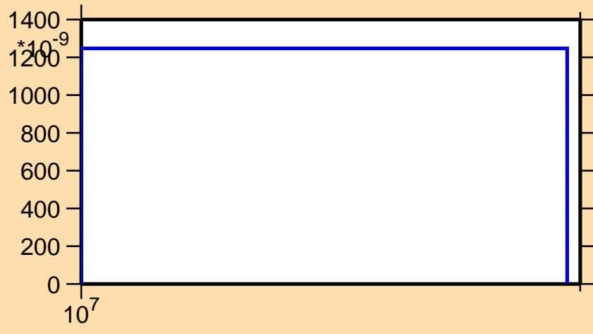
\sigma vs. E for ^{72}\text{Zn}(n,t)
