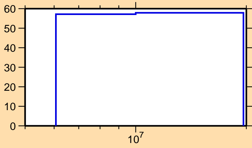
\Delta\sigma/\sigma vs. E for ^{72}\text{Zn}(n,p)
