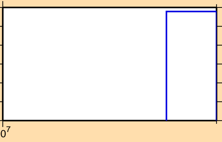
\sigma vs. E for ^{73}\text{Zn}(n,nt)
