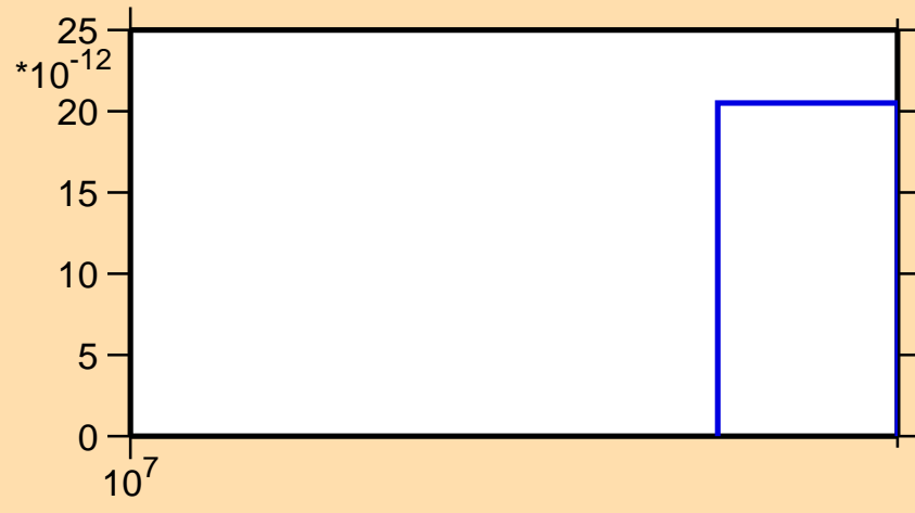
\sigma vs. E for ^{73}\text{Zn}(n,2np)
