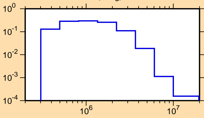
\sigma vs. E for ^{73}\text{Zn}(n,n_3)
