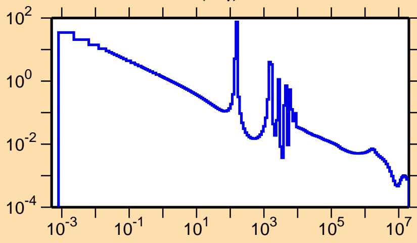
\sigma vs. E for ^{73}\text{Zn}(n,\gamma)
