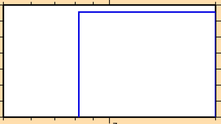
\sigma vs. E for ^{73}\text{Zn}(n,d)
