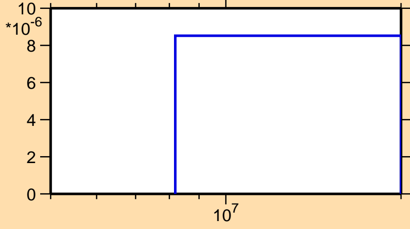
\sigma vs. E for ^{74}\text{Zn}(n,d)
