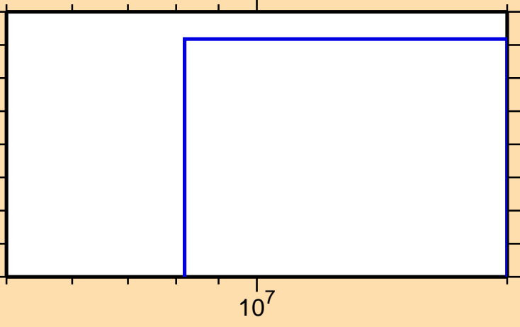
\sigma vs. E for ^{74}\text{Zn}(n,3n)
