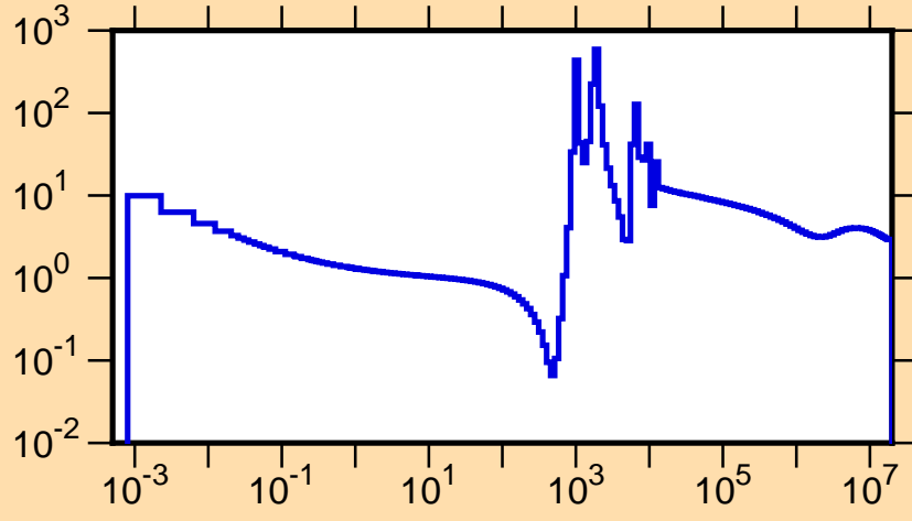
\sigma vs. E for ^{75}\text{Zn}(n,\text{tot.})
