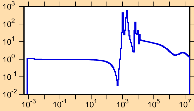
\sigma vs. E for ^{75}\text{Zn}(n,\text{el.})
