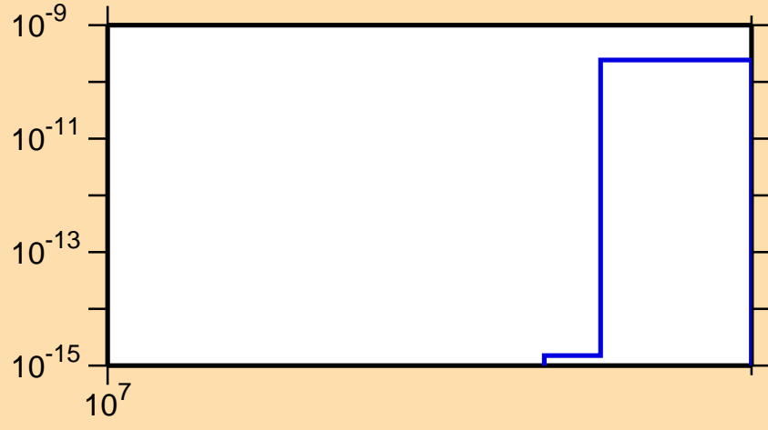
\sigma vs. E for ^{75}\text{Zn}(n,2n\alpha)
