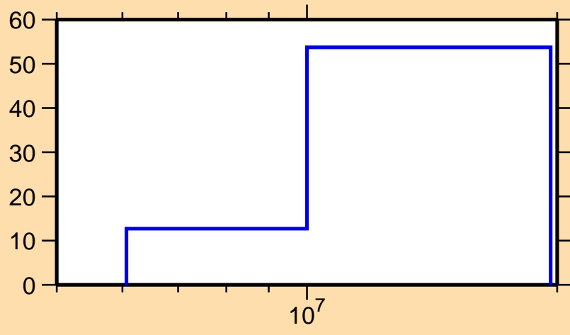
\Delta\sigma/\sigma vs. E for ^{75}\text{Zn}(n,el.)
