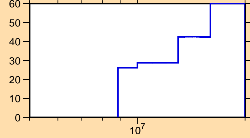
\Delta\sigma/\sigma vs. E for ^{76}\text{Zn}(n,\text{el.})
