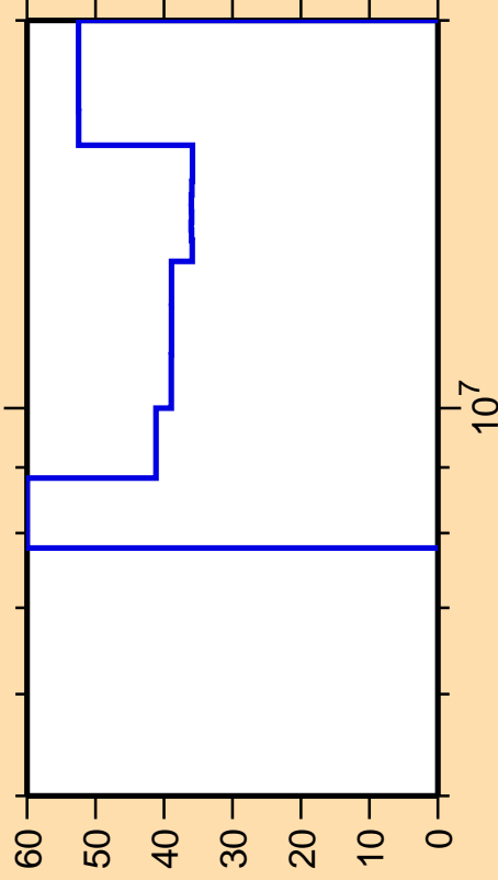
\Delta\sigma/\sigma vs. E for ^{76}\text{Zn}(n,2n)
