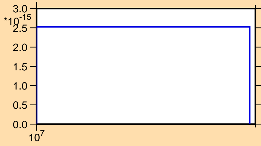
\sigma vs. E for ^{76}\text{Zn}(n,nt)
