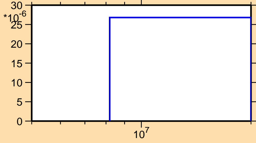
\sigma vs. E for ^{76}\text{Zn}(n,p)
