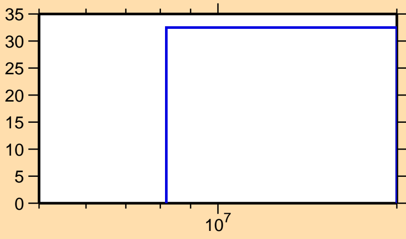
\Delta\sigma/\sigma vs. E for ^{76}\text{Zn}(n,el.)
