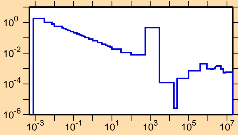
\sigma vs. E for ^{76}\text{Zn}(n,\gamma)
