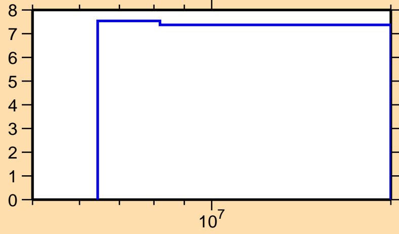
\Delta\sigma/\sigma vs. E for ^{76}\text{Zn}(n,\text{nonel.})
