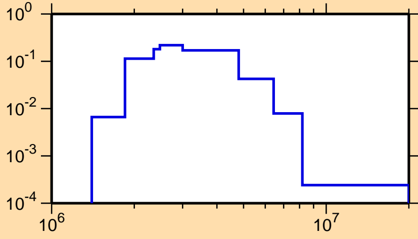
\sigma vs. E for ^{76}\text{Zn}(n,n_4)
