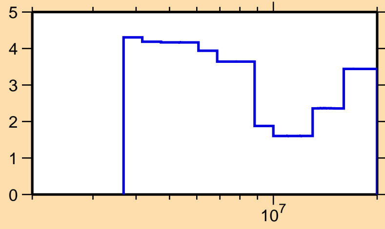
\Delta\sigma/\sigma vs. E for ^{77}\text{Zn}(n,n\text{onel.})
