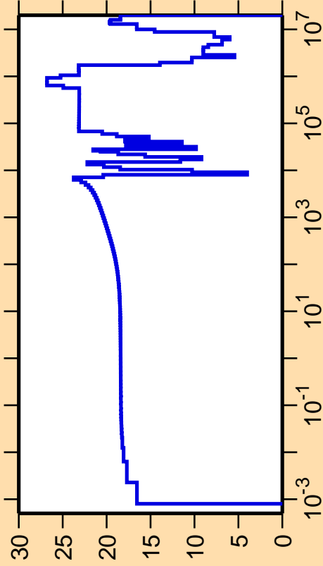
\sigma vs. E for ^{77}\text{Zn}(n,\text{el.})
