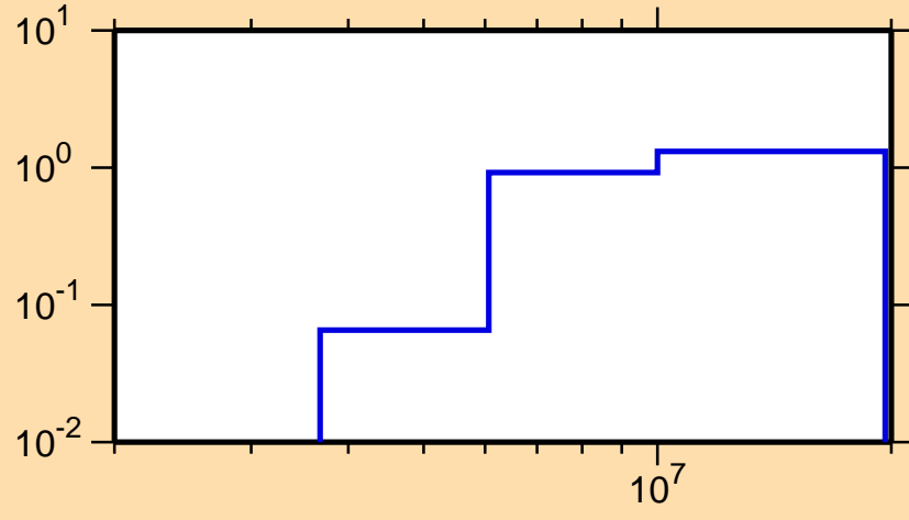
\sigma vs. E for ^{77}\text{Zn}(n,2n)
