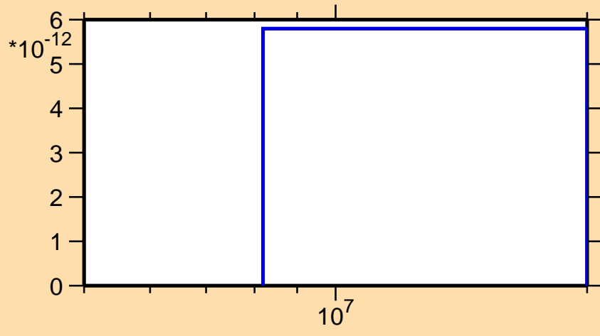
\sigma vs. E for ^{77}\text{Zn}(n,nd)
