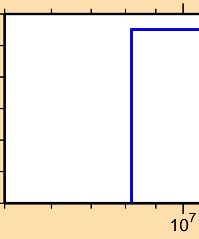
\sigma vs. E for ^{77}\text{Zn}(n,2n\alpha)
