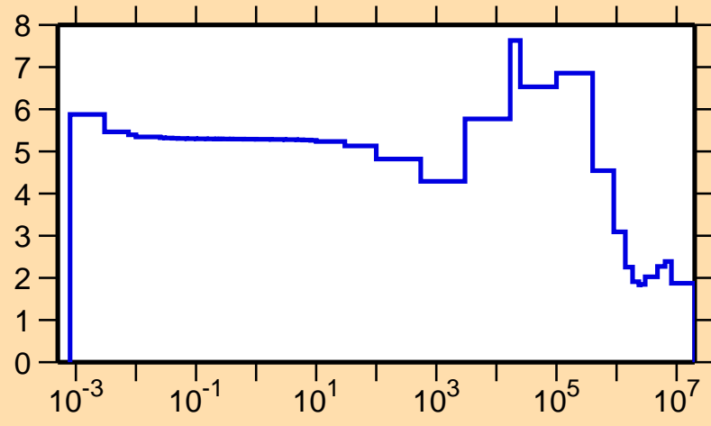
\sigma vs. E for ^{77}\text{Zn}(n,\text{el.})
